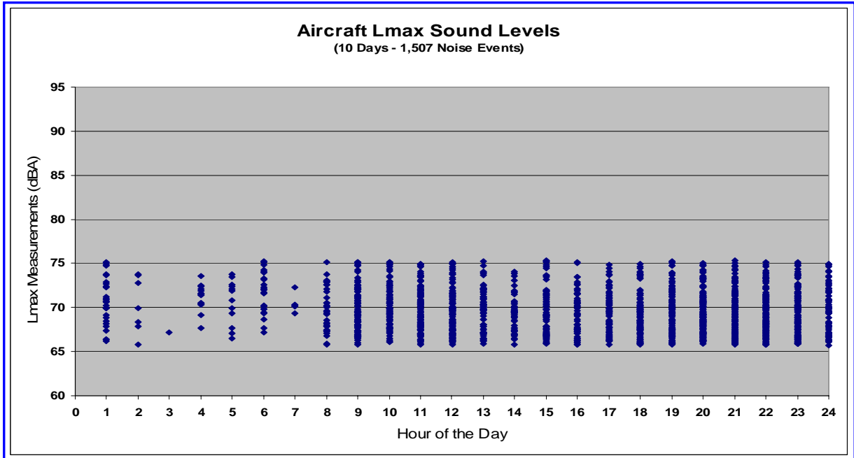
Figure 6. Aircraft Lmax Levels by Hour-of-the-Day
